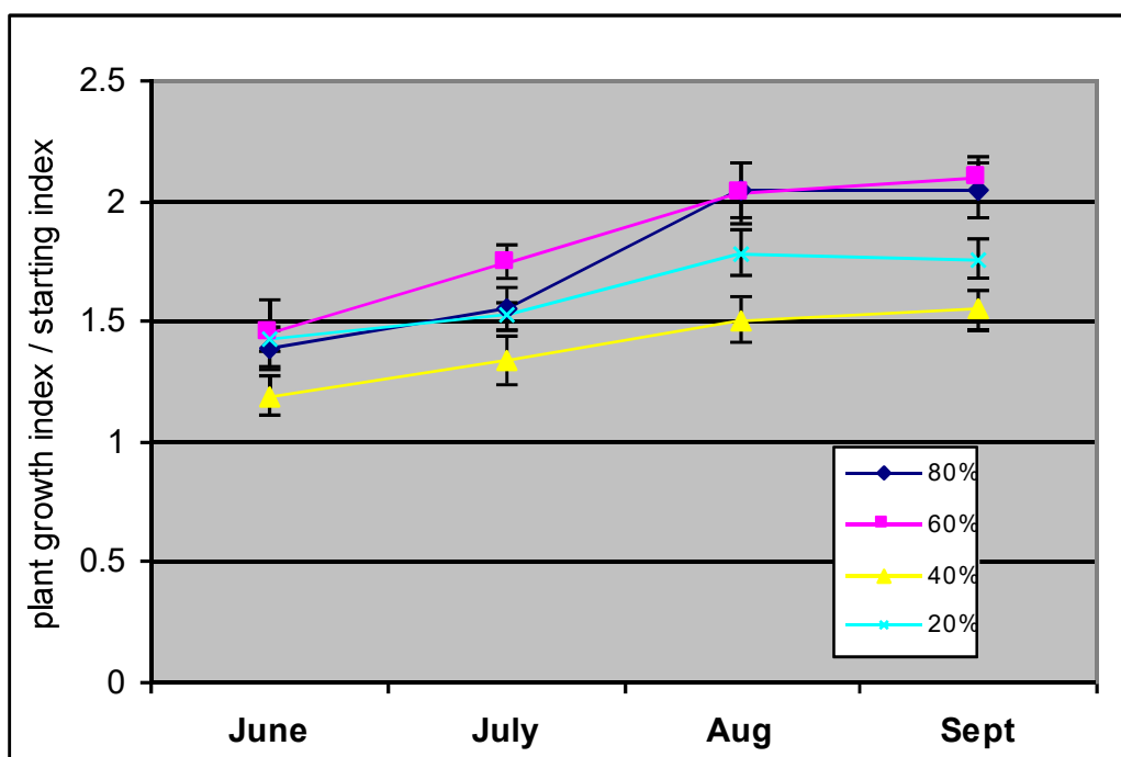
Figure 5b. San Diego sedge relative summer growth
