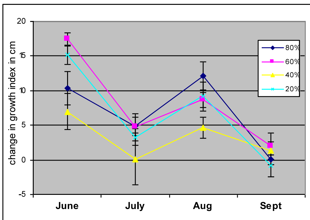
Figure 5a. San Diego sedge summer growth index under 4 irrigation percentages of ETo
