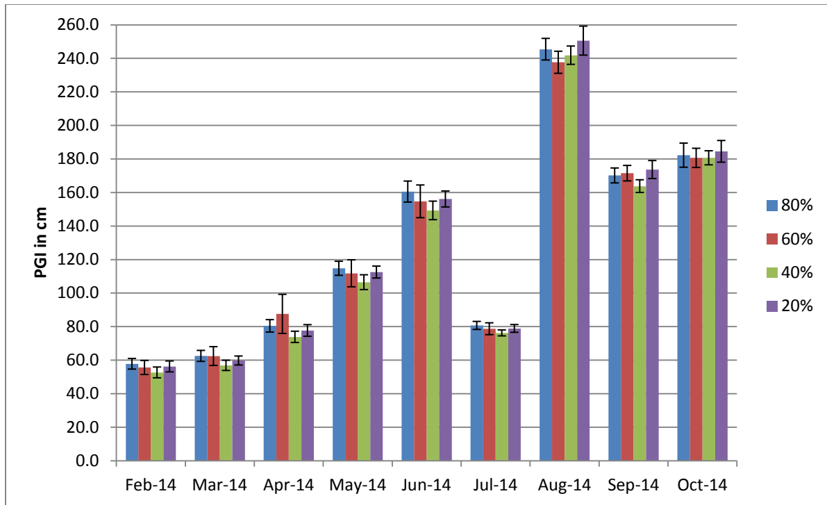
Figure 1. Plant growth index in cm for Kurapia on 4 levels of ET_0 -based irrigation Error bars represent \pm 1 SE; no sig. differences at p \leq 0.05 using ANOVA and Tukey's HSD
