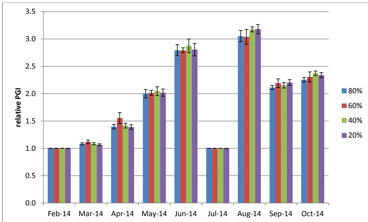
Figure 2. Relative plant growth index for Kurapia on 4 levels of ET_0 -based irrigation Error bars represent \pm 1 SE; no sig. differences at p \leq 0.05 using ANOVA and Tukey's HSD
