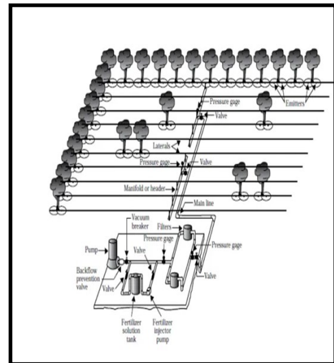
Figure 2. Schematic showing orchard irrigation system beginning with the well and pumping plant and extending out to the last lateral line and sprinkler or
