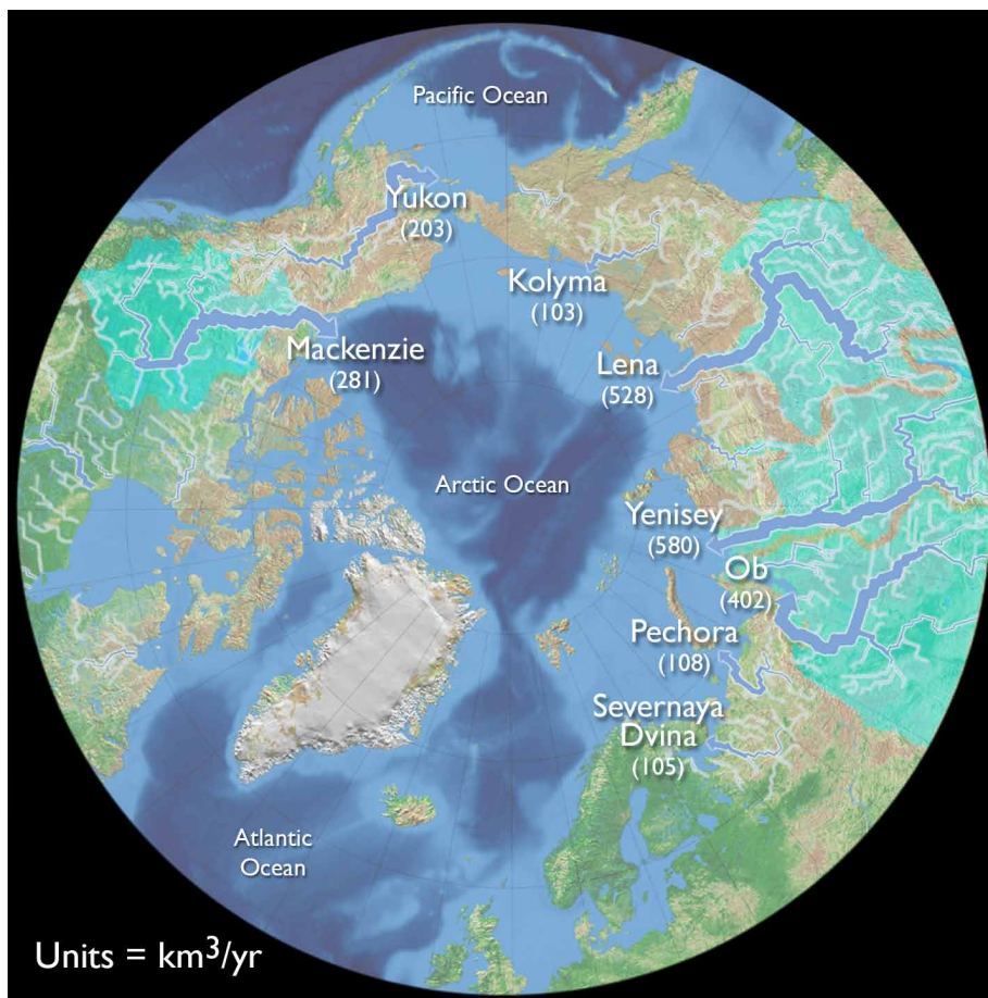
Figure 10 Relative flow contributions to the Arctic Ocean (discharge in cubic kilometres per year).
