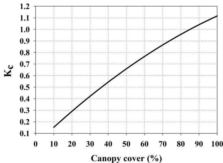
Fig. 3. Relationship between canopy cover (%) and the crop coefficient (K c ); calculation is K_c = (0.63 + 1.5C - 0.0039C^2)/100 , where C is the percent canopy cover.
