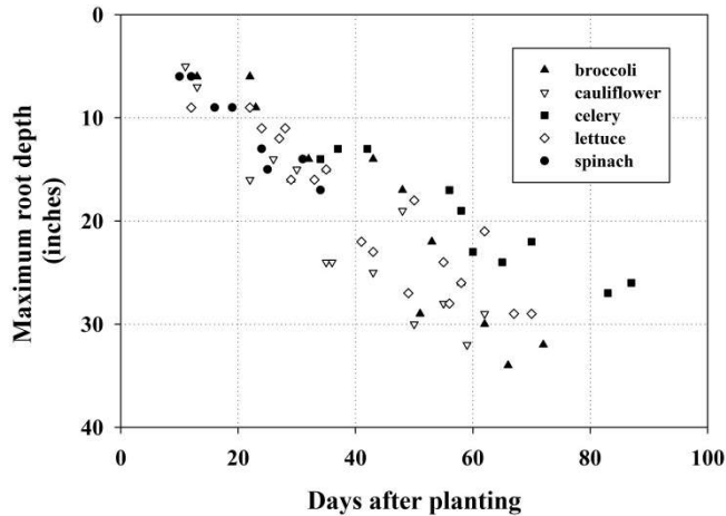
Fig. 2. Pattern of root development in cool-season vegetable crops under summer coastal conditions; data represent the deepest root observed on each evaluation date.
