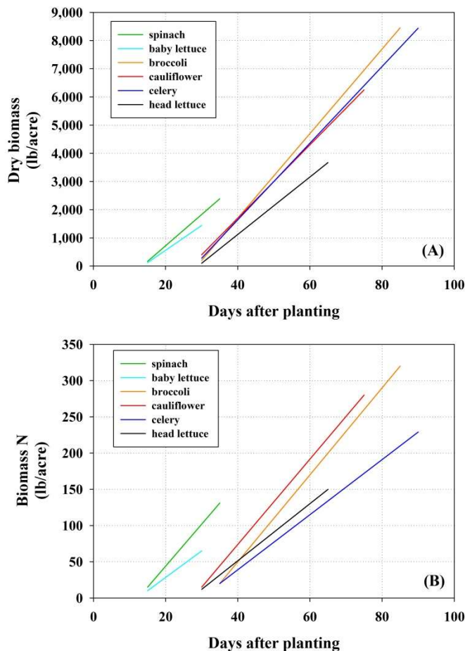
Fig. 1. Pattern of seasonal growth (A) and N uptake (B) by cool-season vegetable crops under summer coastal conditions.
